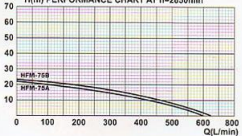
H(m) PERFORMANCE CHART AT n=2850min -1
